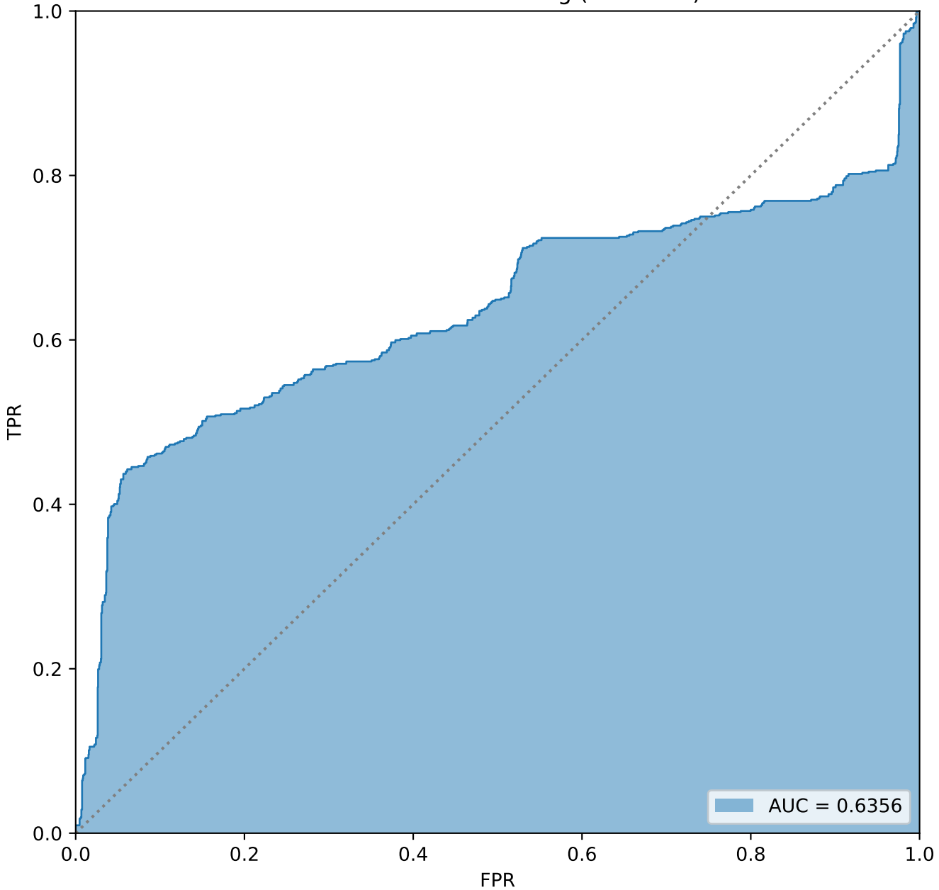
Basic frame differencing (absmean)
