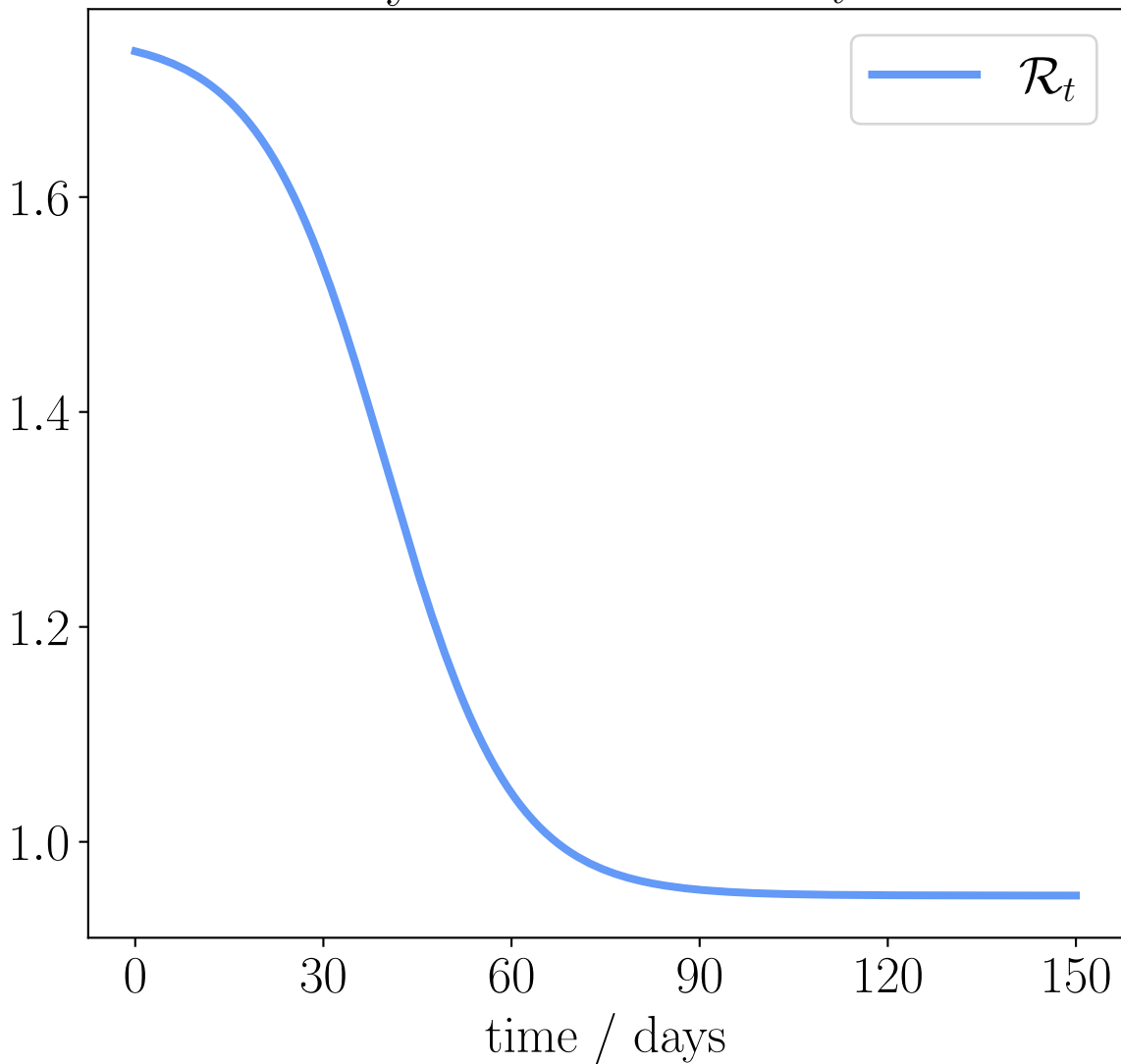
synthetic I data \mathcal{R}_t
