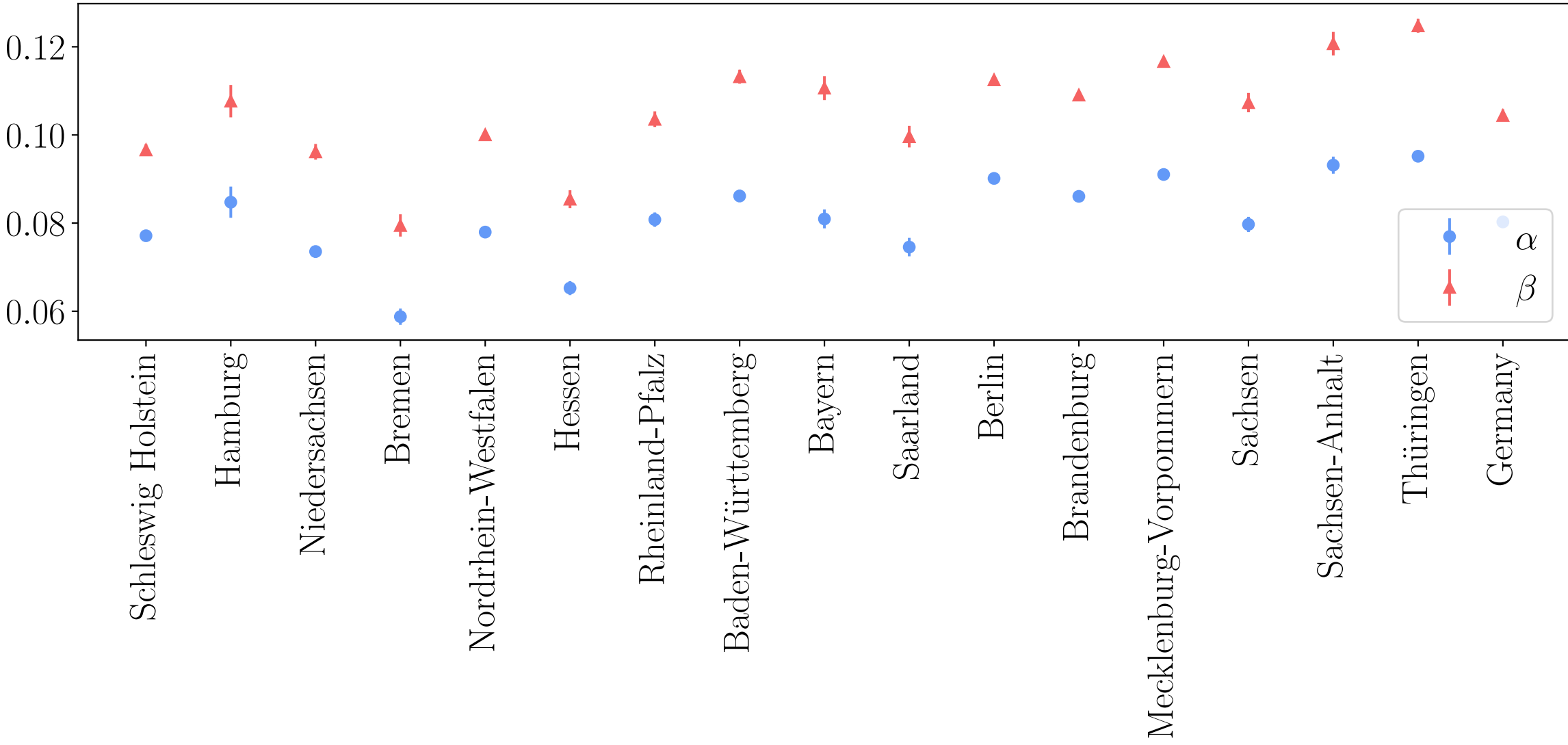
Mean and Standard Deviation
