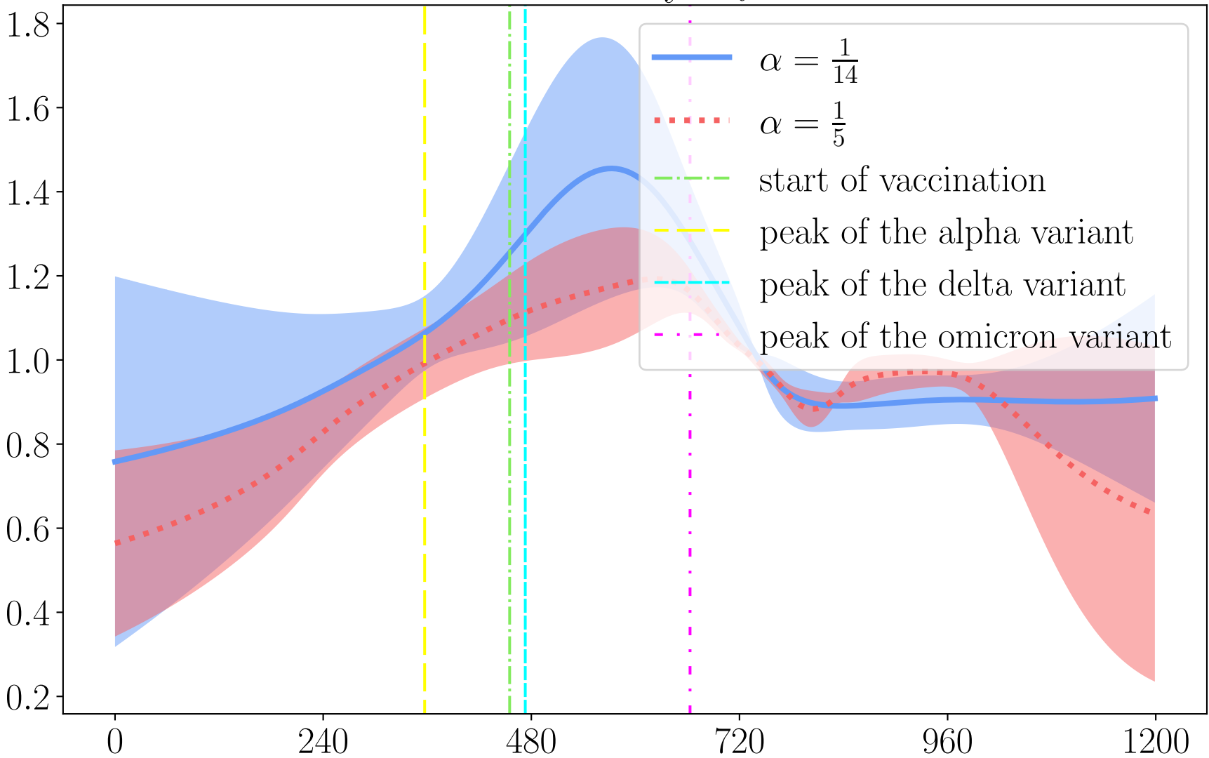
Germany \mathcal{R}_t
